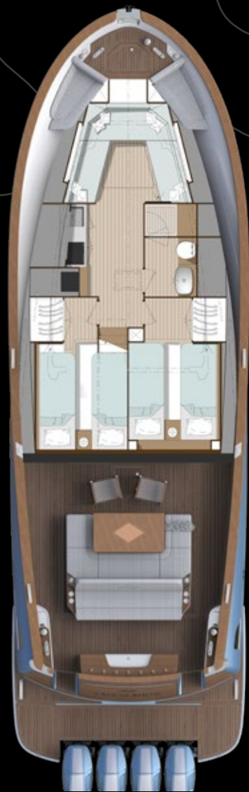
Lowerdeck Lounge Cruise / Two Cabins + Dinette
